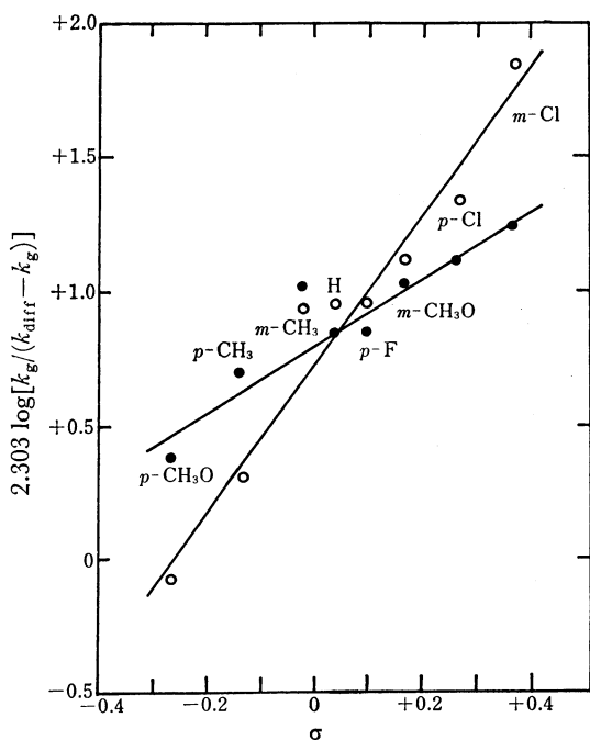
Fig. 4. Linear free-energy relation of the quenching constant: (O) in benzene and (●) in acetonitrile.
